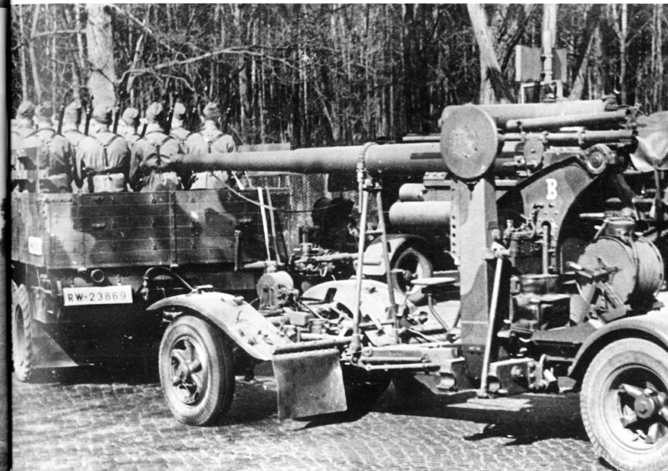
A Henschel truck with a full complement of flak crew inside tows an 8.8cm heavy anti-aircraft gun. Even during the Western Campaign the 8.8cm flak gun demonstrated outstanding anti-tank capabilities and attributed greatly to the success of the Panzer divisions.
