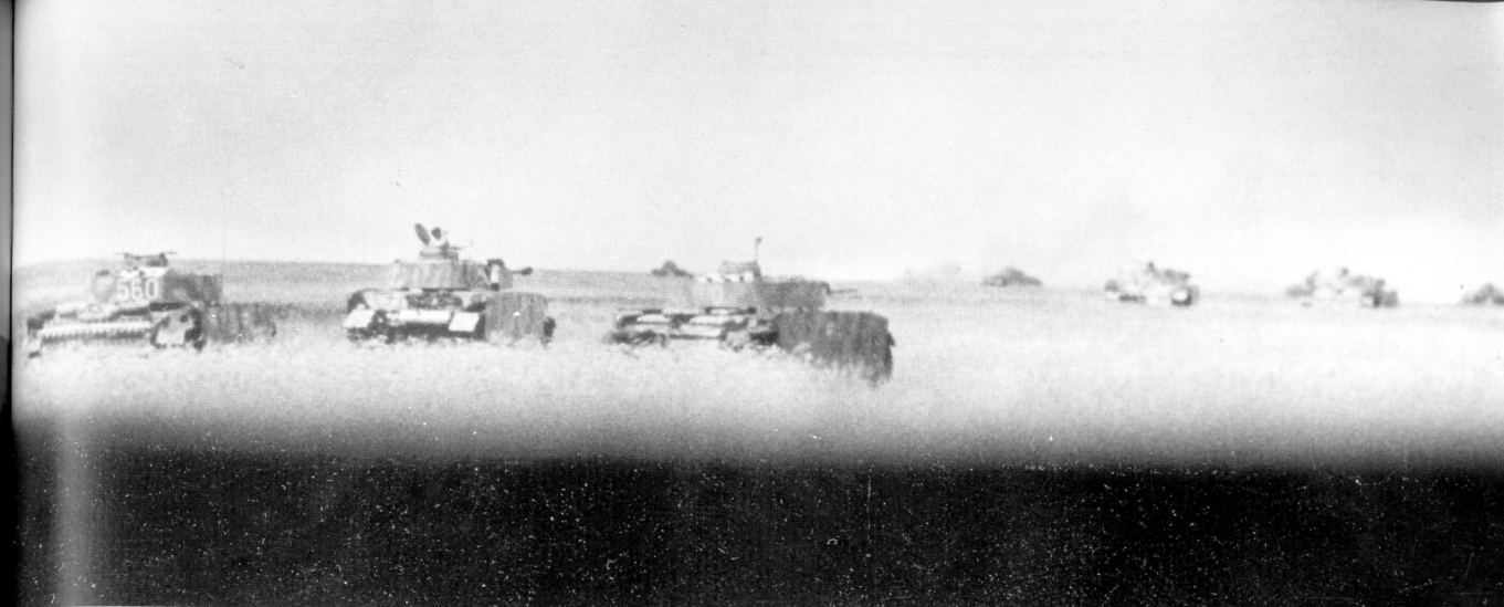
Late version Pz.Kpfw.IV's open fire on Red Army targets during the Kursk offensive, code-named Zitadelle. Note the side skirts or schürzen . The vehicle's protective skirts were made of mild steel plates and were designed to protect the tank from rounds fired at close range by Russian anti-tank fire.
