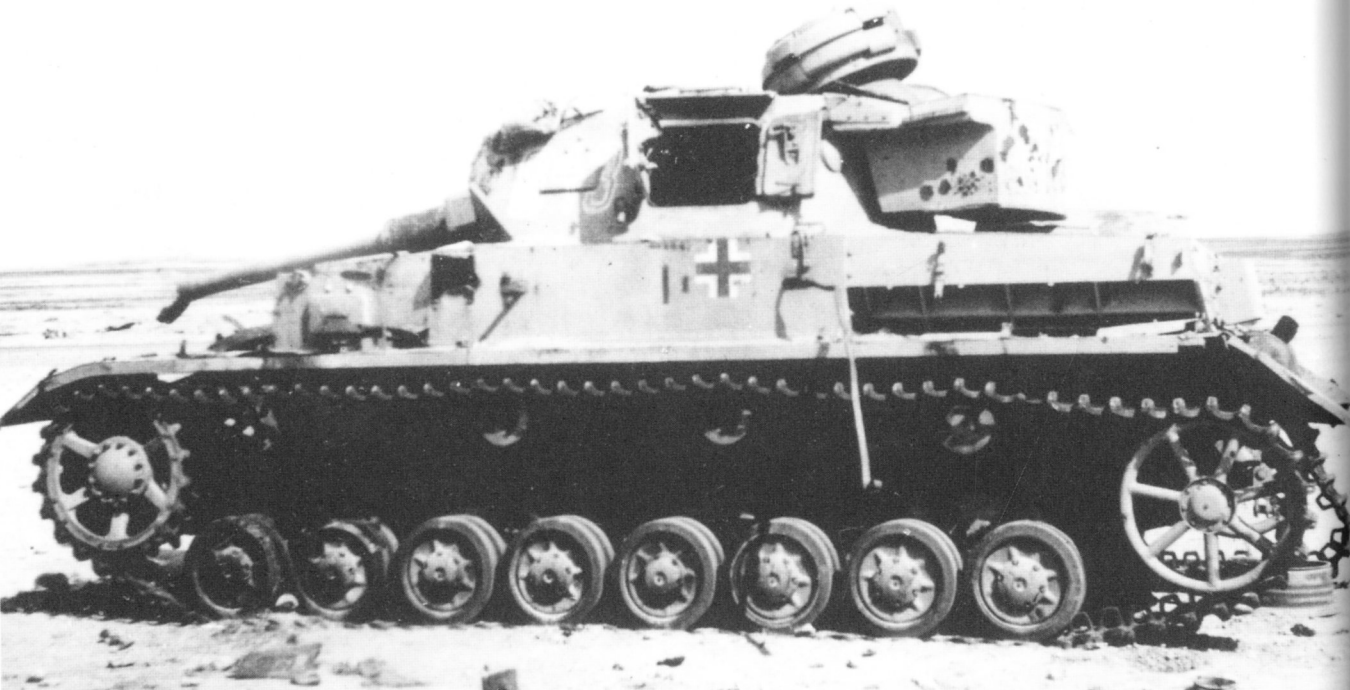
A knocked out Pz.Kpfw.IV in the desert in early 1943. This is just one of many hundreds of destroyed and abandoned vehicles of the once vaunted Afrika-Korps. The Pz.Kpfw. had been used as the main striking force in the Panzer divisions against the British.
